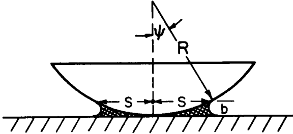
FIGURE 1 Liquid bridge between lens and flat plane.
